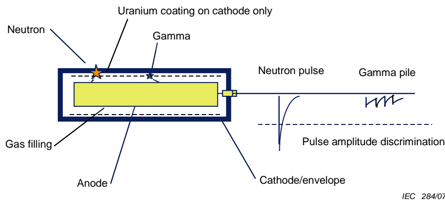
Figure 4 – Diagram of a fission counter
