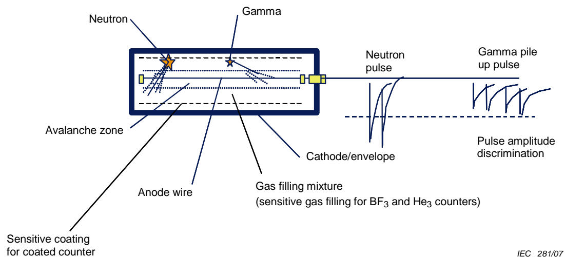
Figure 1 – Neutron sensitive proportional counter
