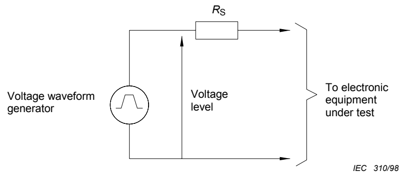
Figure 2a - Test circuit
