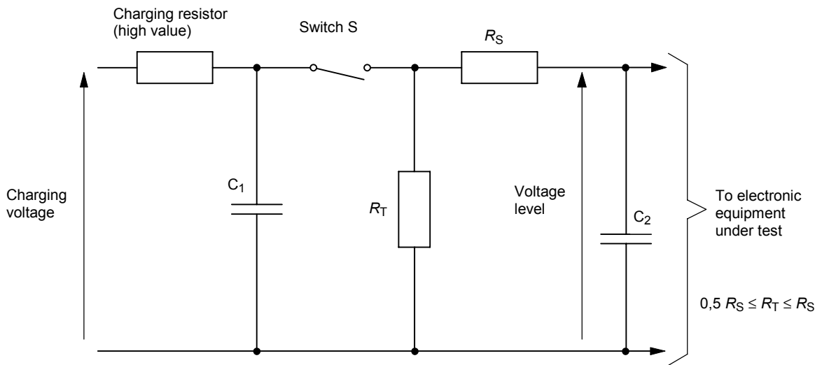
Figure 4a - Test circuit
