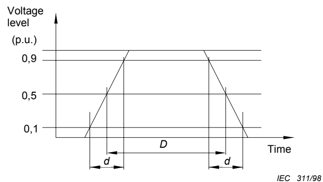
Figure 2b - Test waveform
