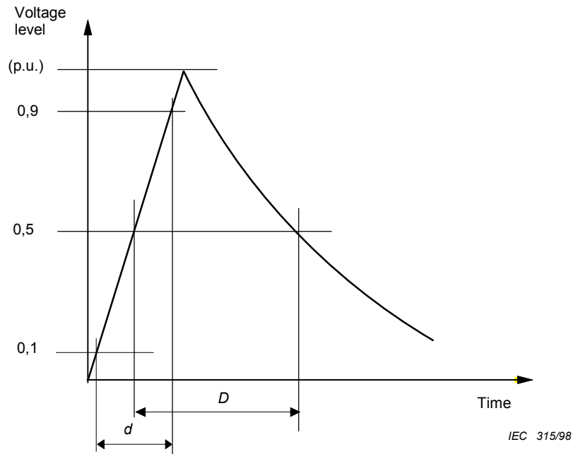
Figure 4b - Test waveform
