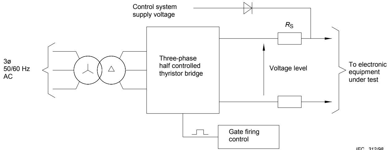
Figure 3a - Typical test circuit
