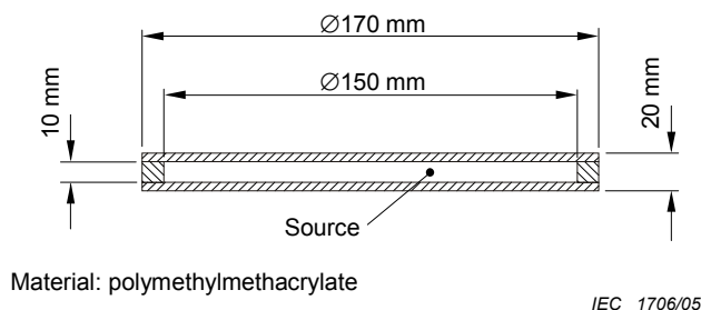
Figure 1 – Cuvette
