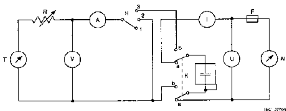
Figure 1 - Circuit to perform the destruction test
