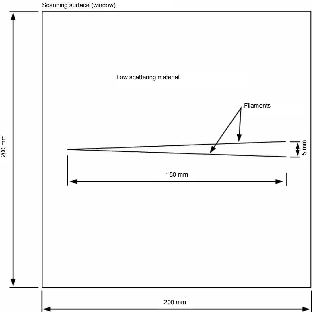
Figure C.2 – Axial resolution test object
