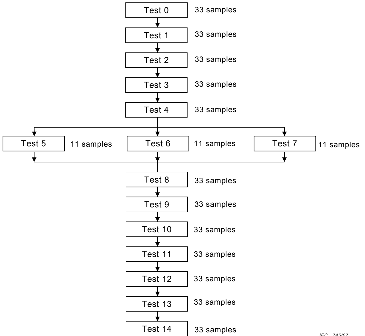
Figure 2 – Reliability qualification tests sequence and grouping required for fibre optic connector sets used in the uncontrolled service environment of Category U
