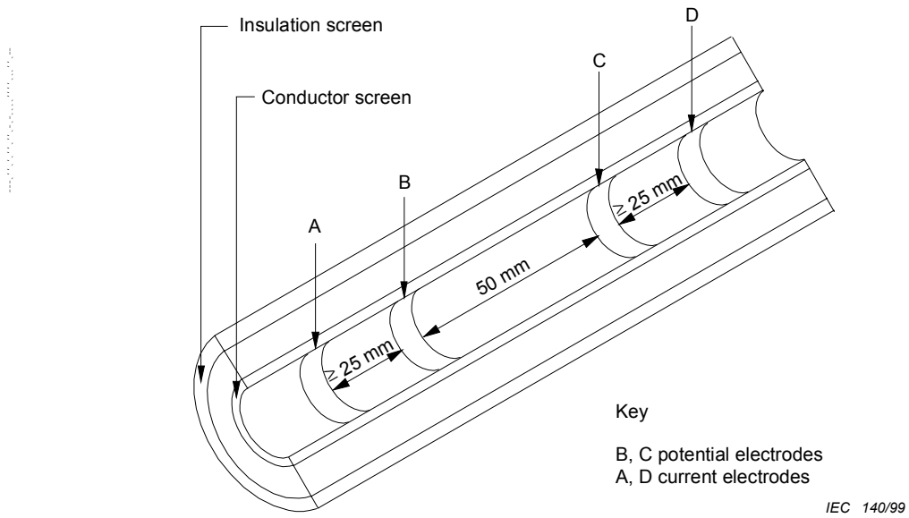
Figure B.1a – Measurement of the volume resistivity of the conductor screen
