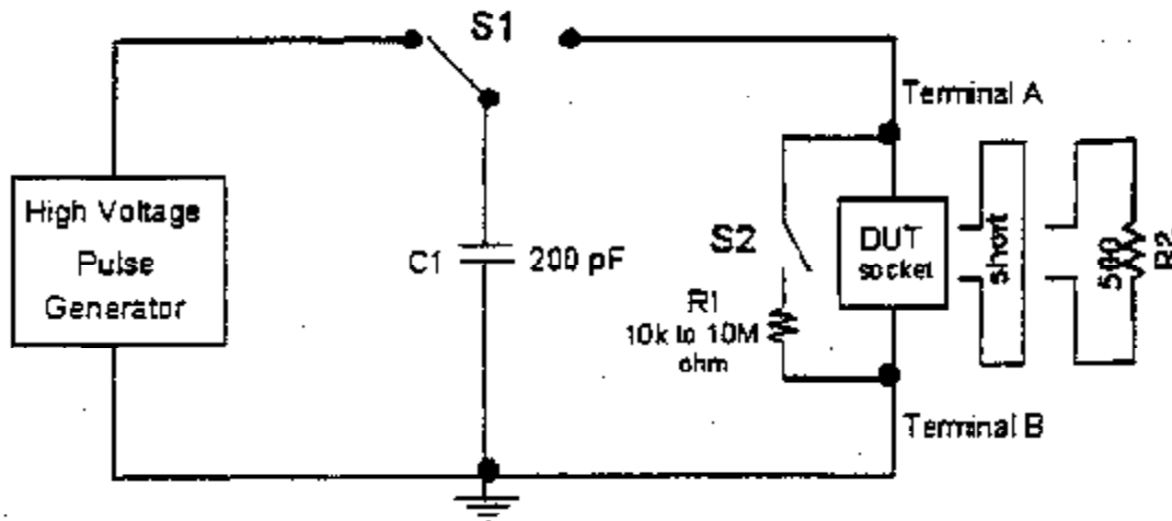
Figure 1 — Typical equivalent MM ESD circuit
