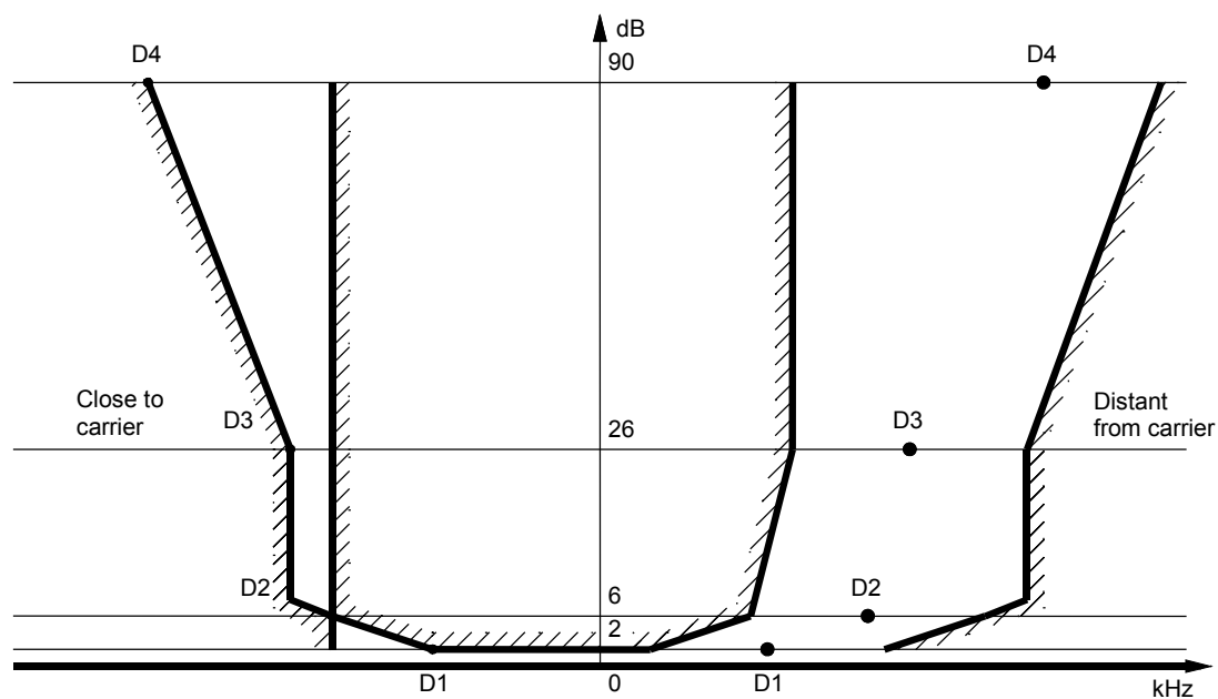
Figure B.1 – IF filter specification
