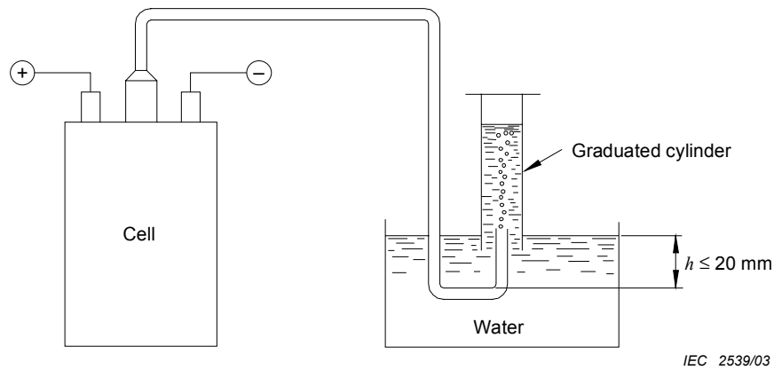
Figure 1 – Method of gas collection
