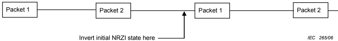
Figure 8 – Format for repeating four-packet cluster
