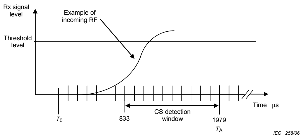
Figure 2 – Carrier-Sense timing
