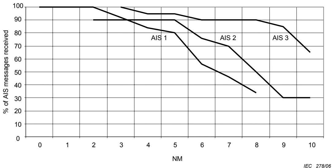
Figure A.4 – Range achieved by a Class A AIS from Class B AIS
