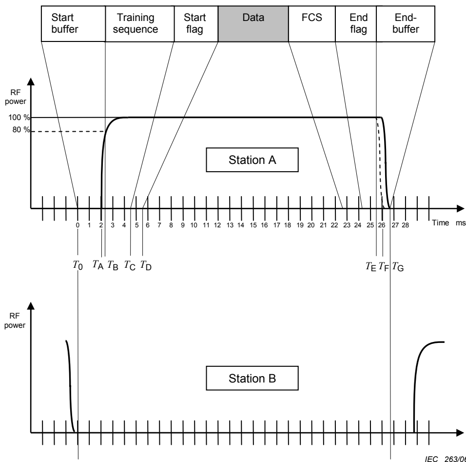
Figure 6 – Transmission timing
