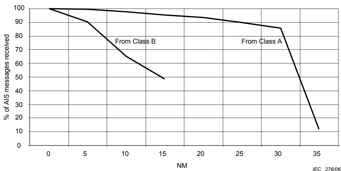
Figure A.2 – Reception of messages by Class A AIS
