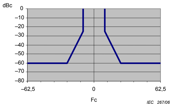
Figure 10 – Emission mask
